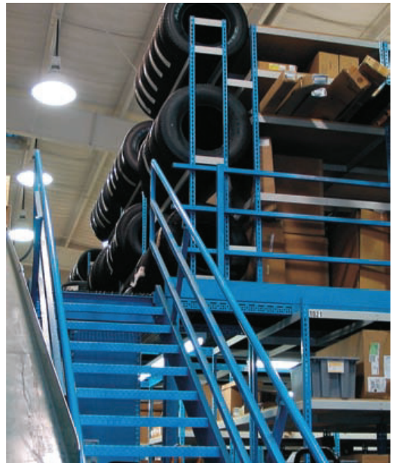
Shelving supported mezzanine with tire racks and long parts storage.
